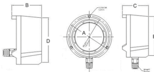
4.5" Bottom Connection with Integral Back Flange
